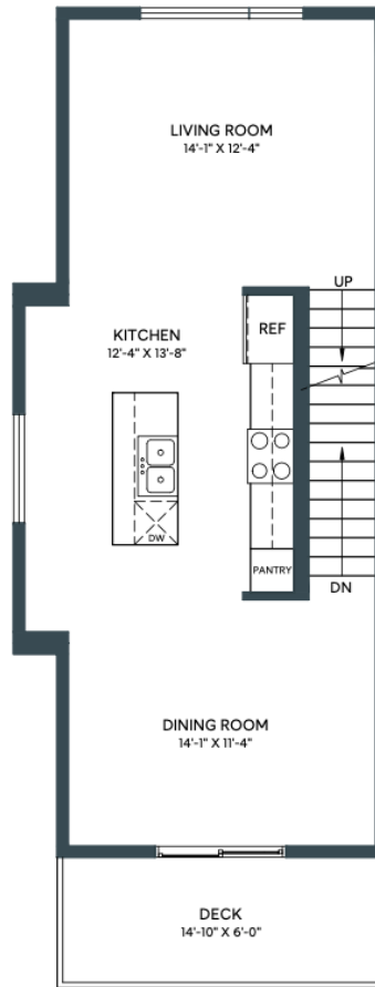
MAIN Second Floor: 619 sq/ft
